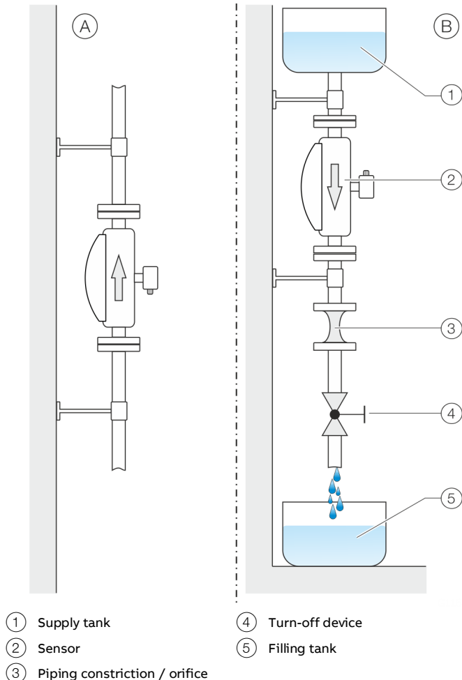
Figure 3: Vertical installation
