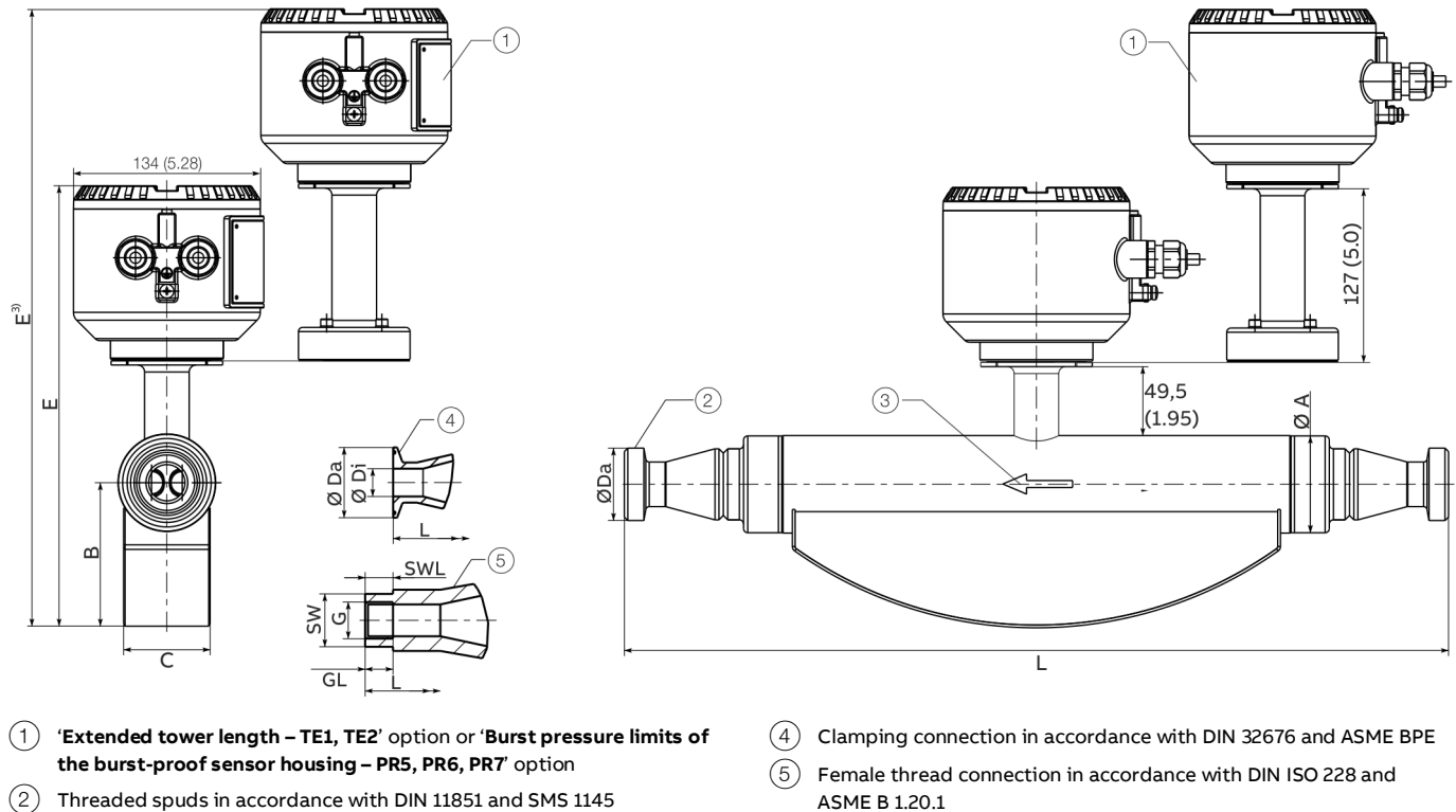
Figure 6: Remote mount design
