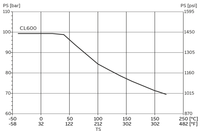
Figure 13: Stainless steel ASME flange 1.4404 (316L) up to DN 200 (8 in.)
