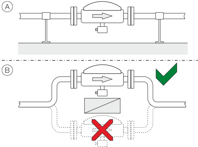
Figure 5: Horizontal installation
