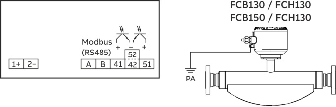
Figure 18: Electrical connection
