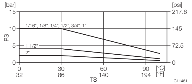
Fig. 11: Material load graph for gas
