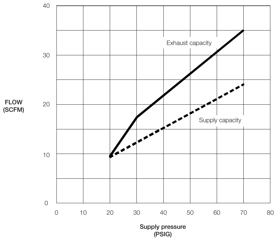
Fig. 2: Capacity (exhaust to atmosphere)
