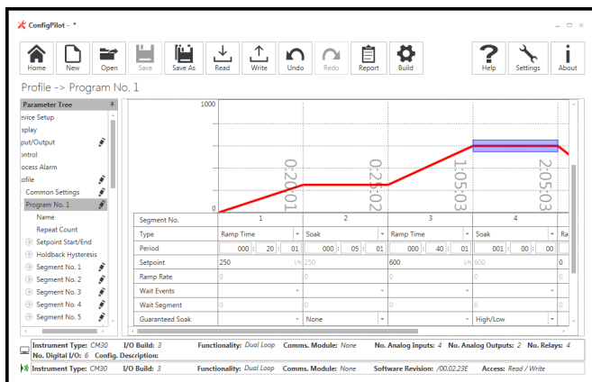
Figure 9 Profile configuration
