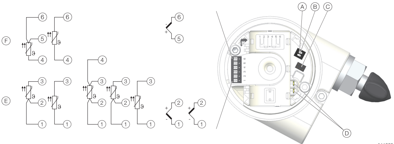
Fig. 9: Electrical connections (opened connection head)
