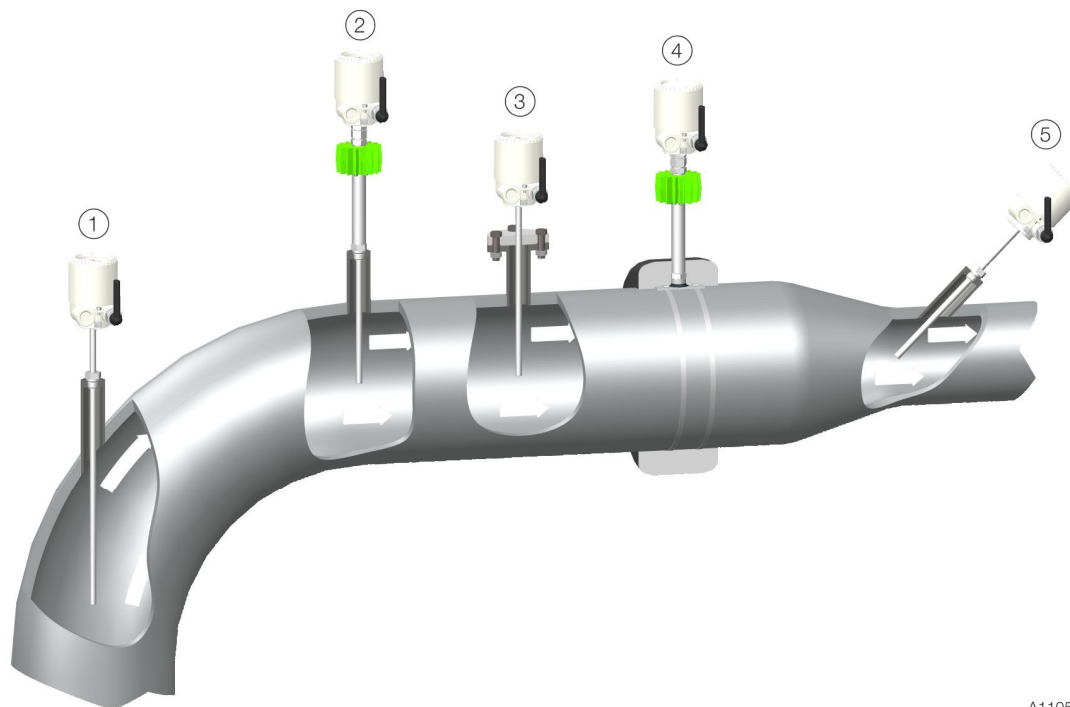
Fig. 5: Installation positions
