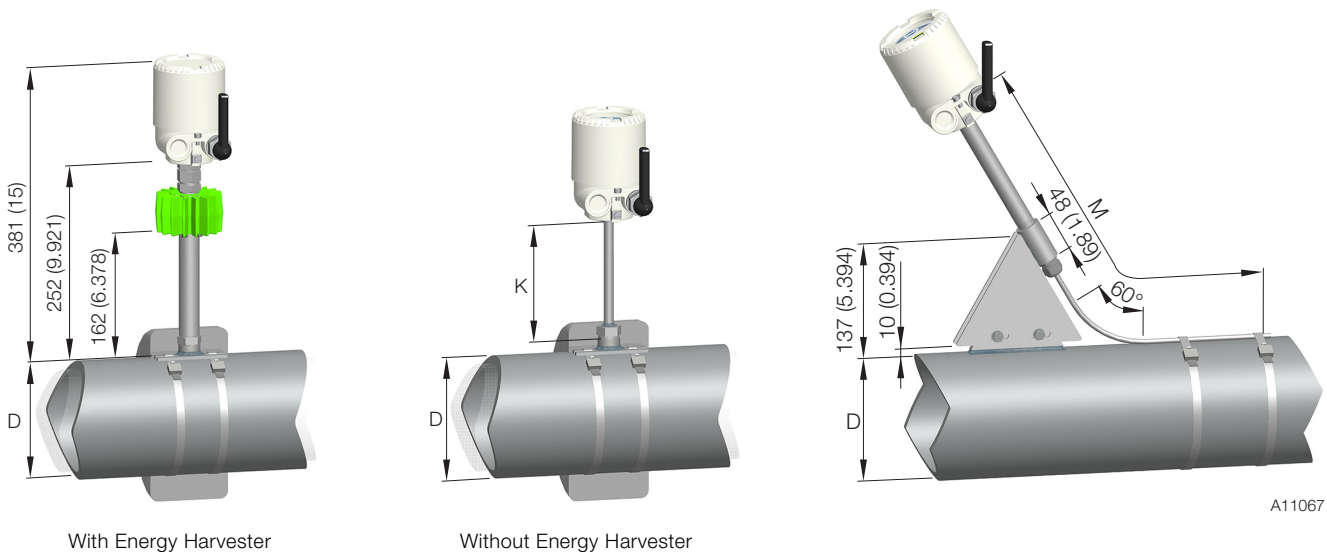
Fig. 8: Sensor fastening 90° to piping / alongside piping
